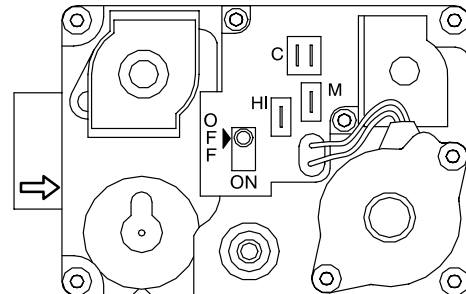
GAS VALVE SHOWN IN OFF POSITION
