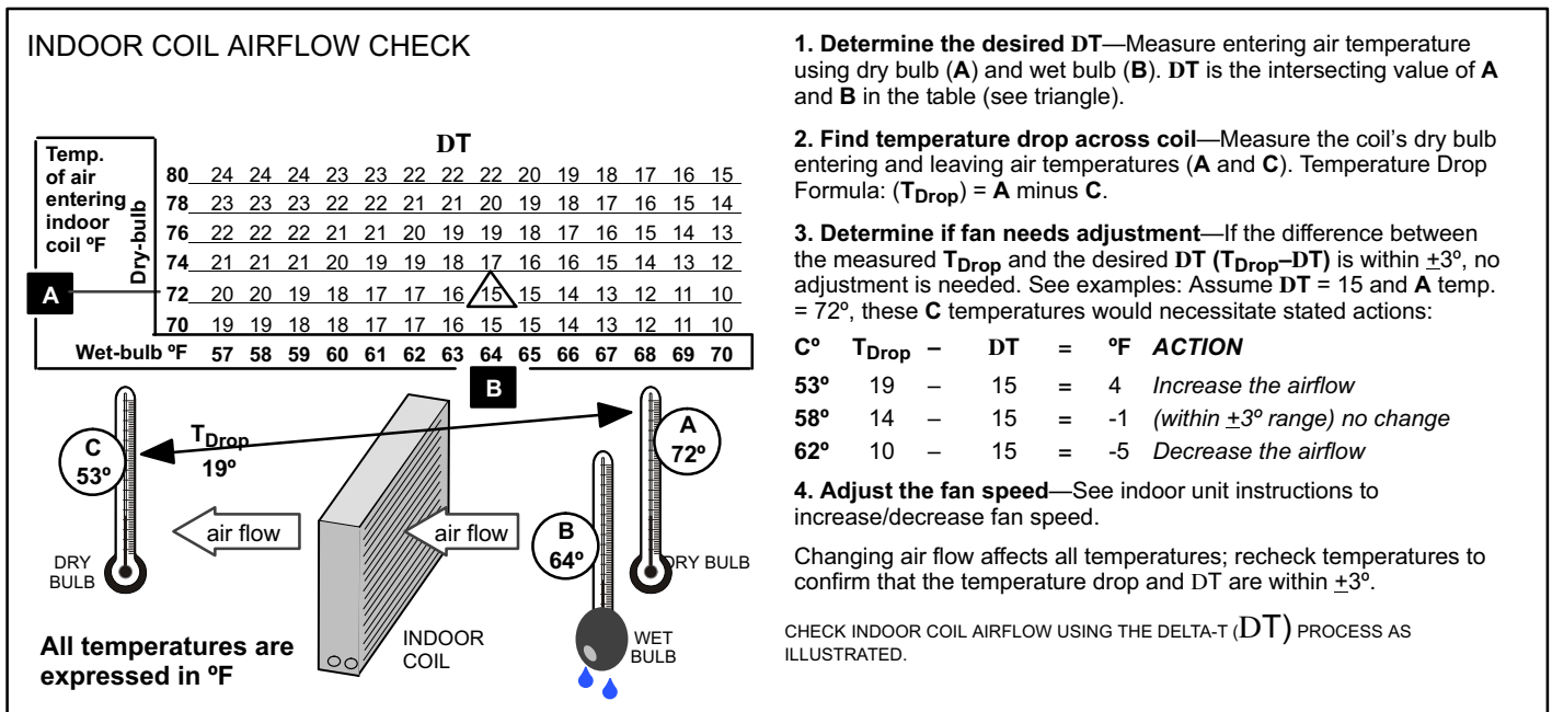
Figure 12. Indoor Coil Airflow Check
